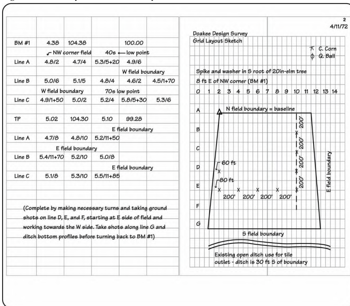
Figure 1-65: Survey Notes—Grid Survey
