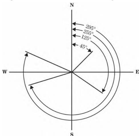
Figure 1-61: Azimuths Showing 0^\circ Oriented to the North
