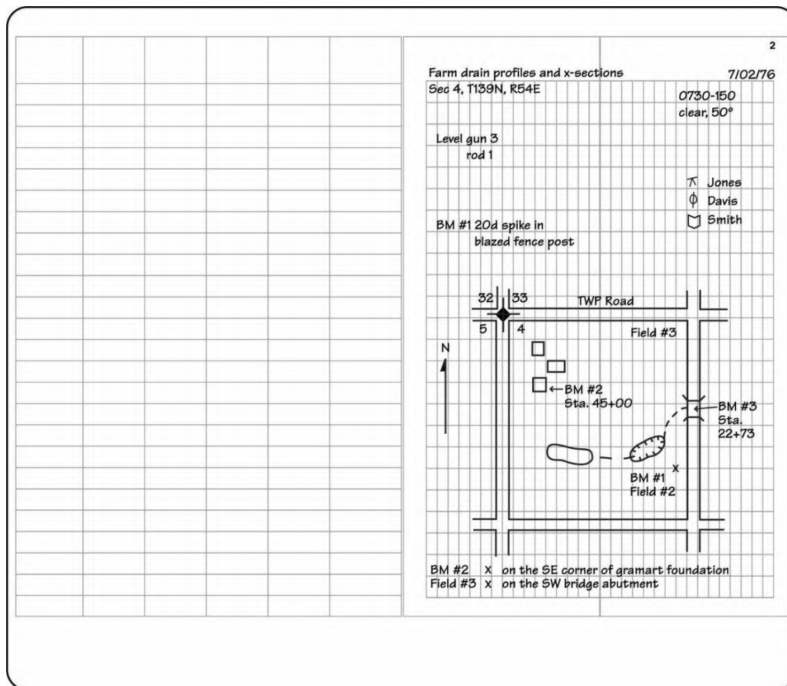
Figure 1-68: Survey Notes—Profile and Cross Section
